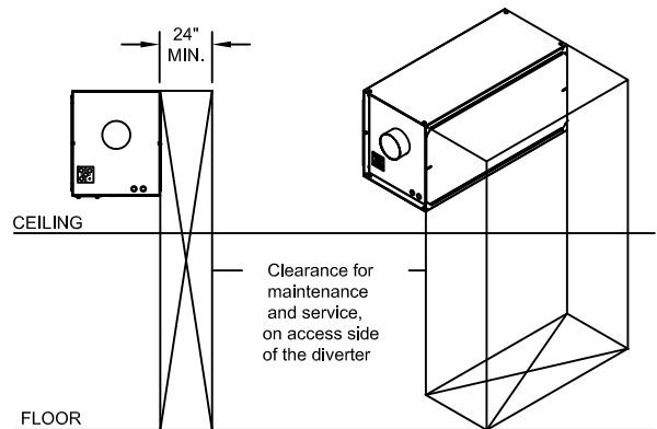
ACCESS CLEARANCE
