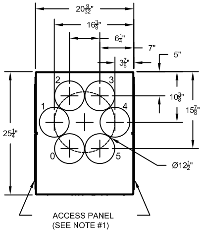
MULTI PORT SIDE UNIT DIMENSIONS
