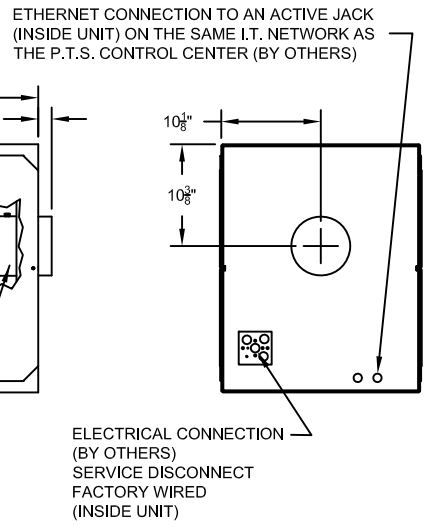
SINGLE PORT SIDE UNIT DIMENSIONS
